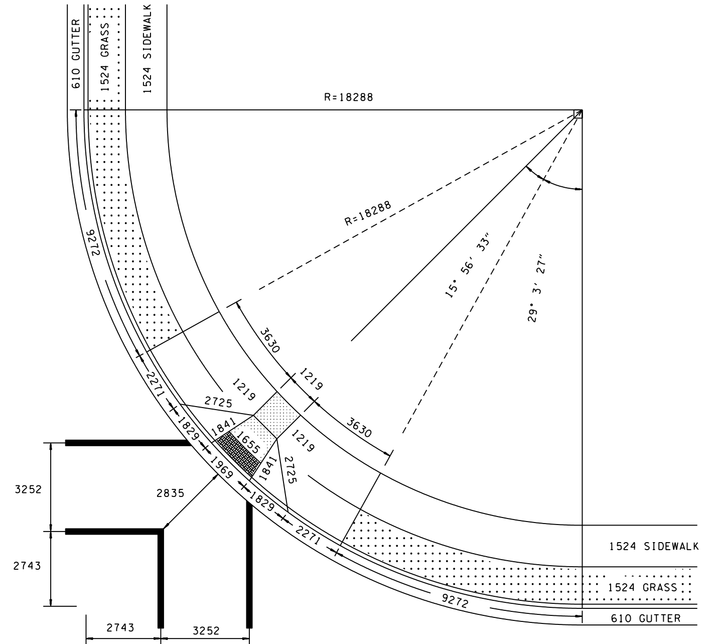
WITH 1524 mm GRASS STRIP R=18288
